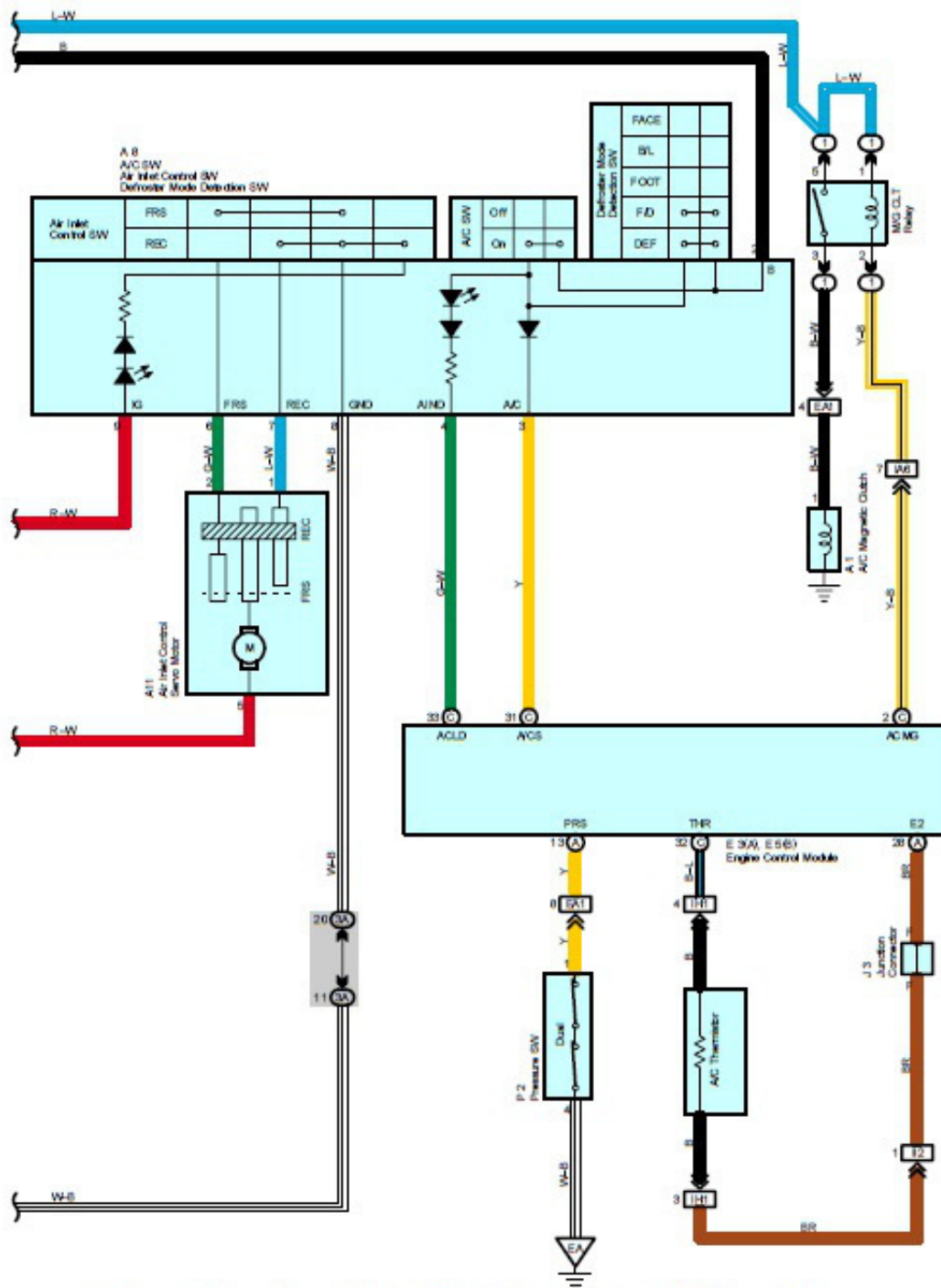
Toyota Corolla Air Conditioning System Wiring Diagram
